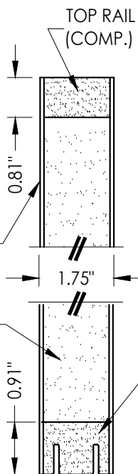
SECTION H-H
