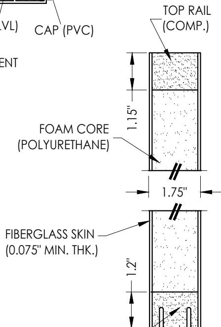
SECTION F-F
