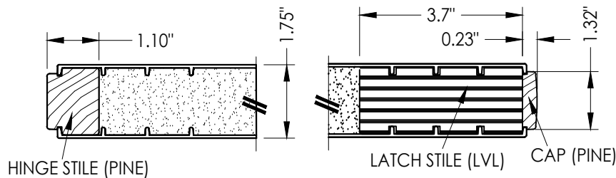
SECTION G-G
