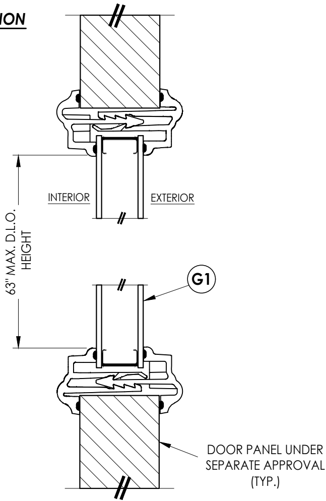
1 2 VERTICAL CROSS SECTION
